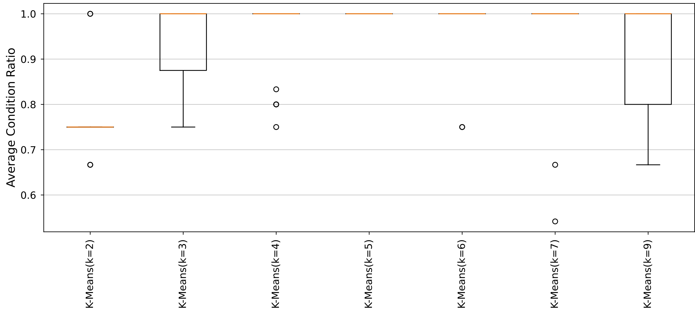
YARA Rules Average Condition Ratio Distribution (Cluster12_Size9 dataset)
